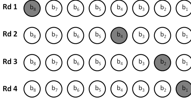
Figure 1: An illustrative example of a sequence of candidate bandits. The incumbent candidate in each round is shaded in grey.
