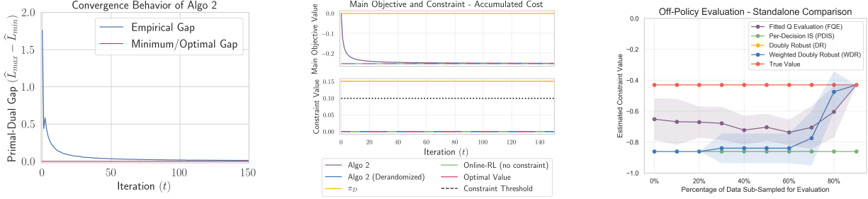
Figure 1. FrozenLake Results . (Left) Empirical duality gap of algorithm 2 vs. optimal gap. (Middle) Comparison of returned policy and others w.r.t. (top) main objective value and (bottom) safety constraint value. (Right) FQE vs. other OPE methods on a standalone basis.
