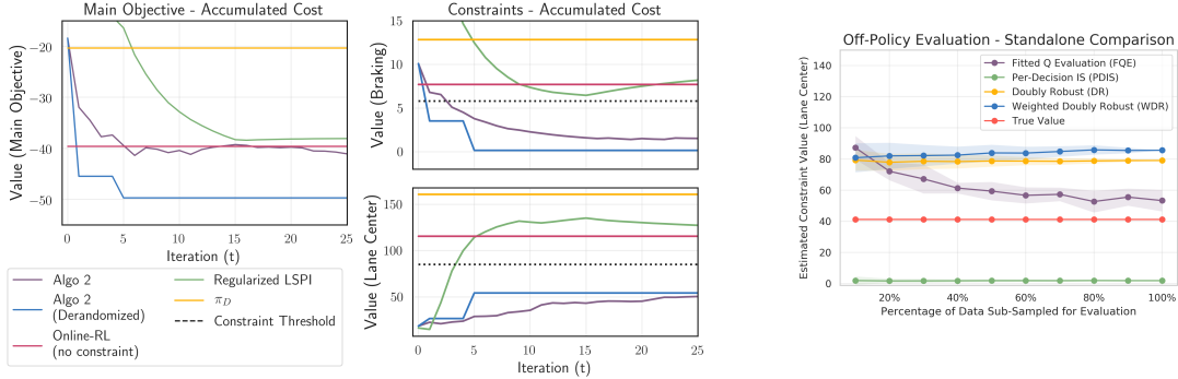
Figure 2. CarRacing Results . (Left) & (Middle) (Lower is better) Comparing our algorithm, regularized LSPI, online RL w/o constraints, behavior policy \pi_D w.r.t. main cost objectives and two constraints. (Right) FQE vs. other OPE methods on a standalone basis.
