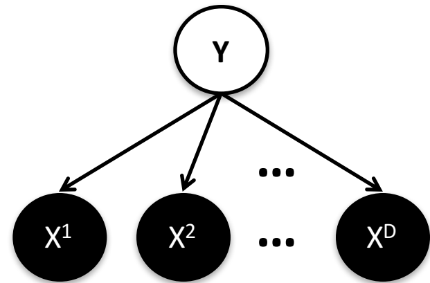
Graphical Model Diagram
